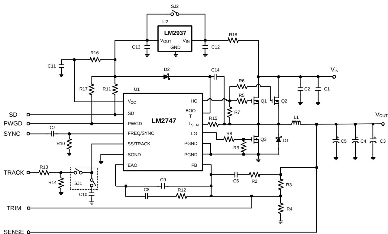
Figure 11. 300 kHz Demo Board Schematic
